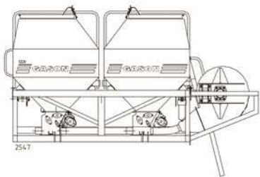
1220 Capacity 2200 L
