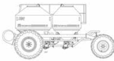
1860RT CTS 2 Bin Capacity 6200 L 3 Bin Capacity 6490 L
