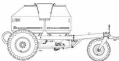
1890RT CTC 2 Bin Capacity 9200 L 3 Bin Capacity 9260 L (non packed)
