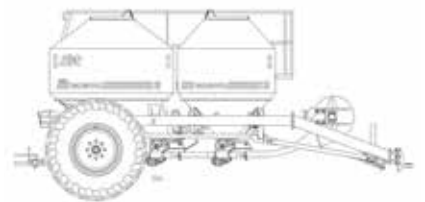
1860FT 2 Bin Capacity 6200 L 3 Bin Capacity 6490 L
